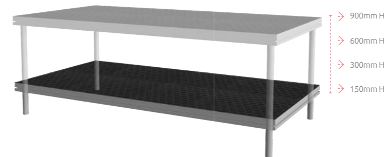
QAS Staging L1220 D2440 | Available in 150mm, 300mm, 600mm, or 900mm H
